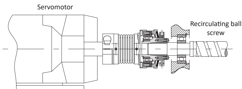
Model DSS/SG/N assembled with bellows coupling GSF between servomotor and recirculating ball screw
