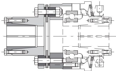
Model DSS/SG with single flexing disc coupling GTR/S for applications where torsional rigidity is required.
