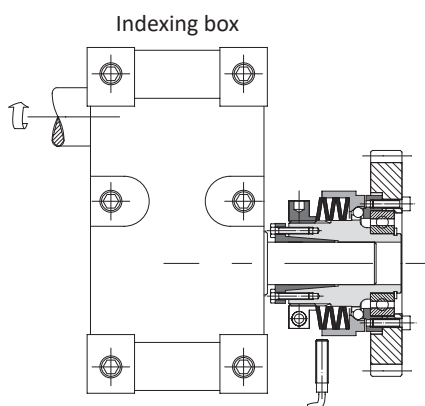
Model DSS/F/SG/P assembled out of the indexing box
